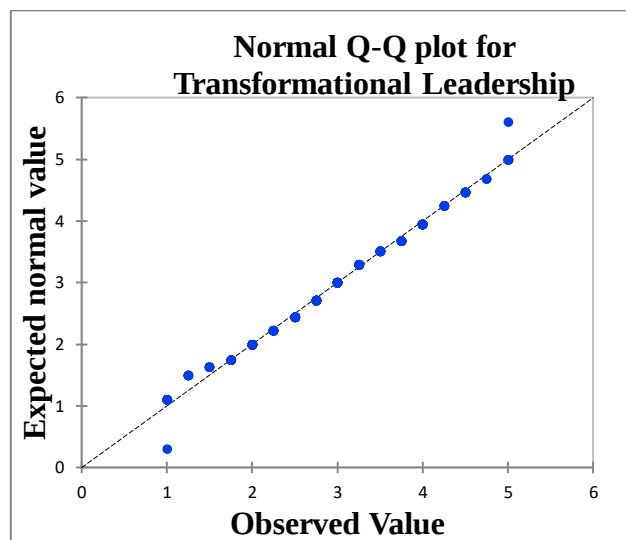
Figure 2: Q-Q Plot of the Dependent Variable
